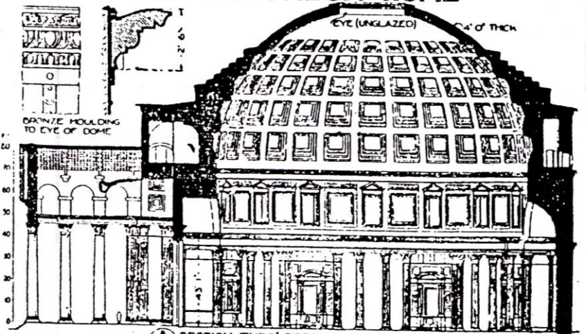
(A) SECTION THRO' PORTICO AND ROTUNDA
